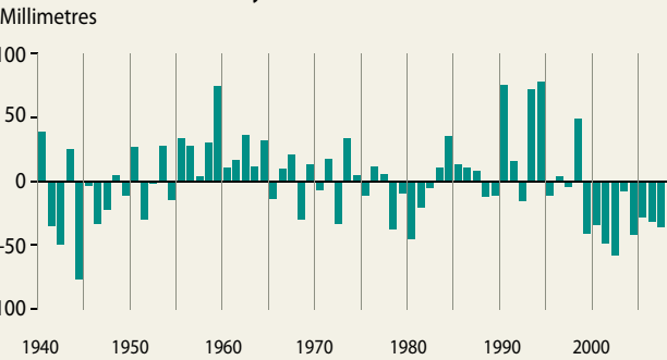
Annual total rainfall anomaly
