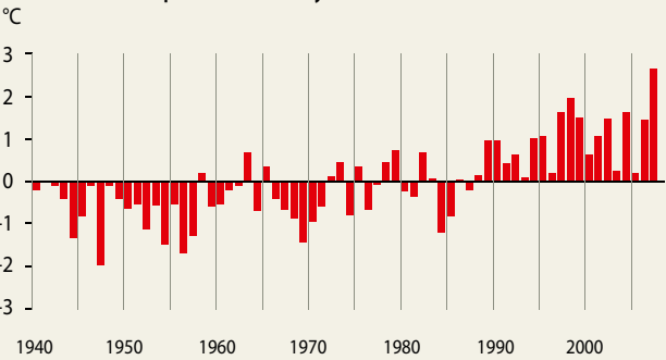
Annual mean temperature anomaly
